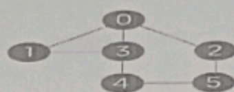
Graph with six nodes
